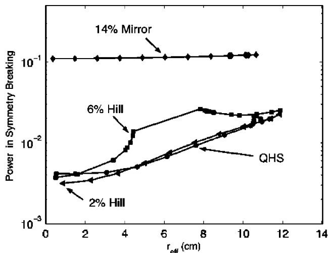
FIG. 4. The fractional power in symmetry breaking spectral components for the four configurations, where the power is defined using Eq. (8).
