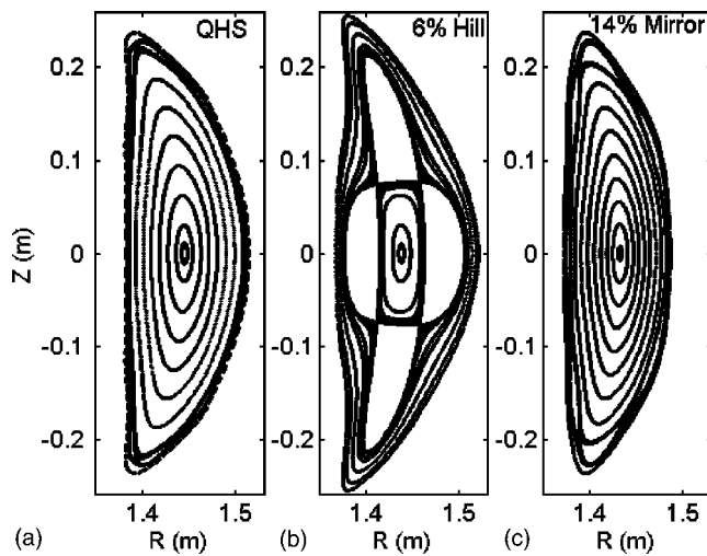
FIG. 2. Magnetic surfaces at the ellipsoidal shaped symmetry plane for the QHS, 6% Hill, and 14% Mirror configurations. The rational surfaces apparent in Fig. 1 appear as gaps between the closed magnetic surfaces in these plots. The surfaces displayed in the calculations are the surfaces on which the Hamada spectrum and damping rates are calculated.
