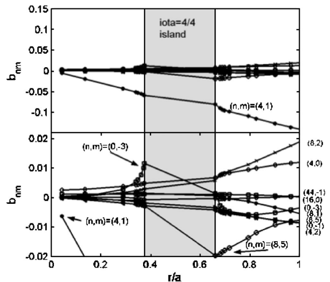
FIG. 3. (a) The complete Hamada spectrum for the 6% Hill configuration and (b) a detailed view of the smaller spectral components. The \iota = 4/4 island chain exists in the shaded region and the spectral components are discontinuous across the gap due to the different magnetic surface shapes on either side of the island. The ten largest spectral components at r/a = 0.372 are illustrated in the plot.
