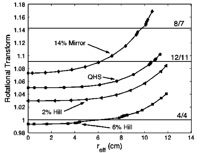
FIG. 1. Rotational transform profiles for the QHS, 2% Hill, 6% Hill, and 14% Mirror configurations. Important low-order resonances are displayed as horizontal lines. These symbols for the different configurations will be maintained throughout this paper.
